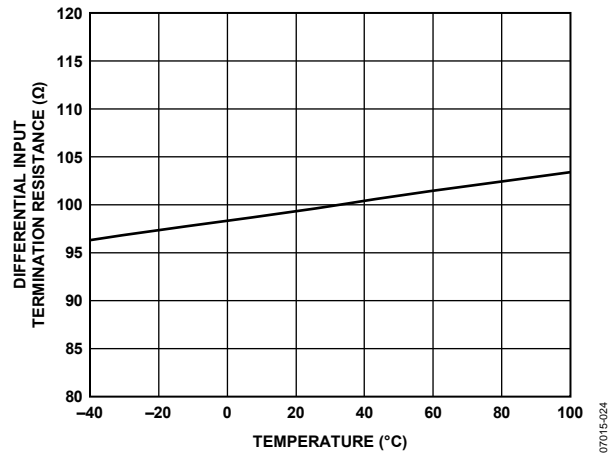
Figure 24. Differential Input Termination Resistance vs. Temperature
