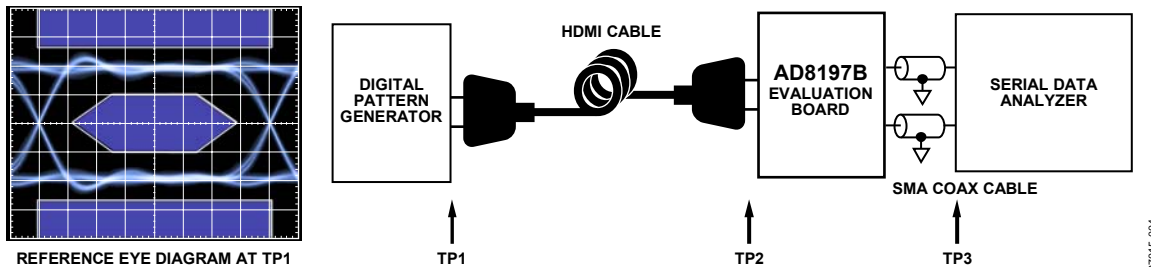
Figure 4. Test Circuit Diagram for Rx Eye Diagram
