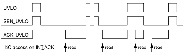
Figure 40. Interrupt Operation Example
