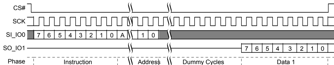
Figure 8.5 RSFDP Command Sequence
