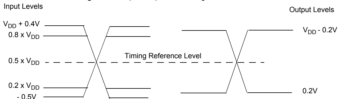
Figure 12.3 Input, Output, and Timing Reference Levels
