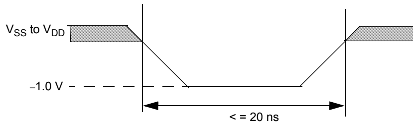
Figure 11.1 Maximum Negative Overshoot Waveform
