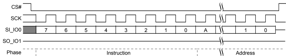
Figure 8.58 Block Erase (BE D8h or 4BE DCh) Command Sequence
