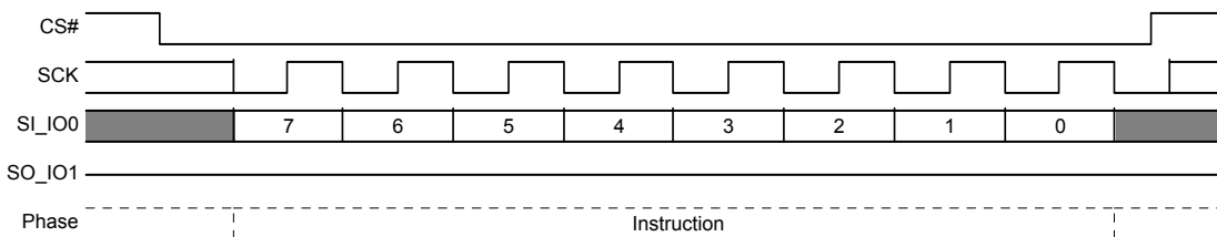
Figure 8.37 Enter QPI Mode (QPIEN 38h) Command Sequence
