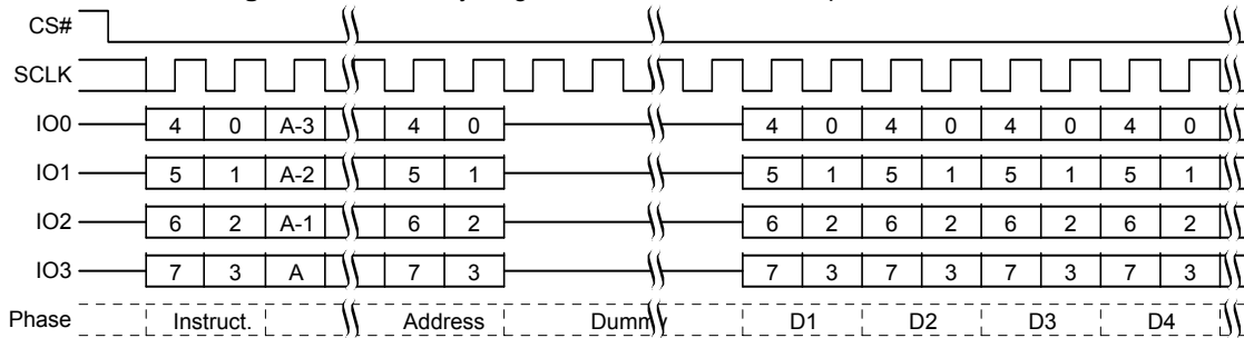
Figure 8.68 Security Regions Read Command Sequence QPI mode
