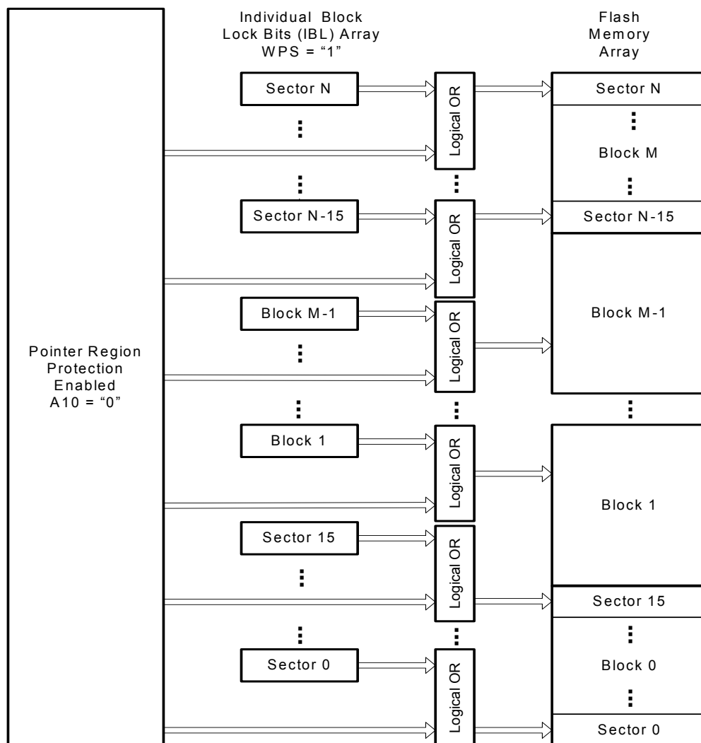
Figure 7.2 Individual Block Lock / Pointer Region Protection Control
