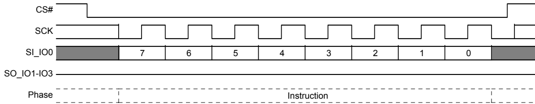
Figure 5.3 Stand Alone Instruction Command
