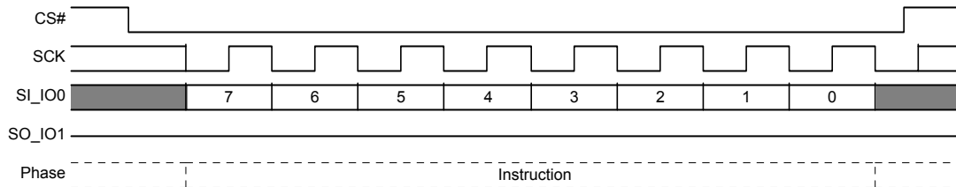
Figure 8.21 Clear Status Register (CLSR) Command Sequence
