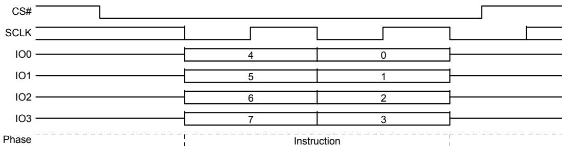
Figure 8.61 Chip Erase Command Sequence QPI Mode
