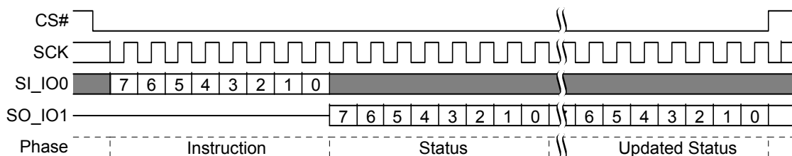
Figure 8.11 Read Status Register 2 (RDSR2) Command
