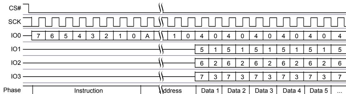
Figure 8.53 Quad Page Program Command Sequence
