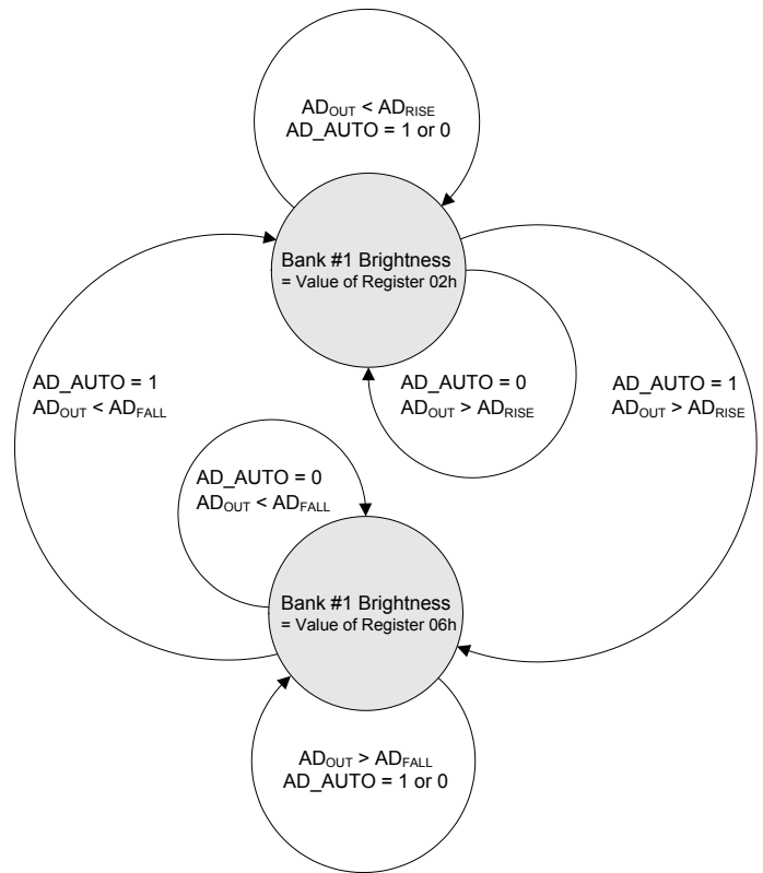
Figure 29 — ADC function at Bank #1 Brightness
