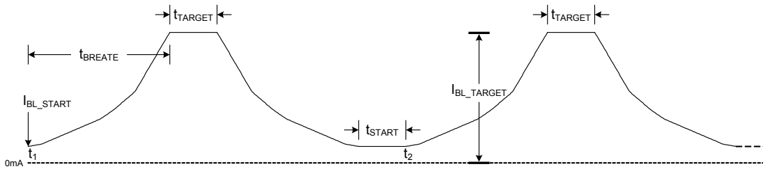
Figure 3 — Breathe Timing Diagram
