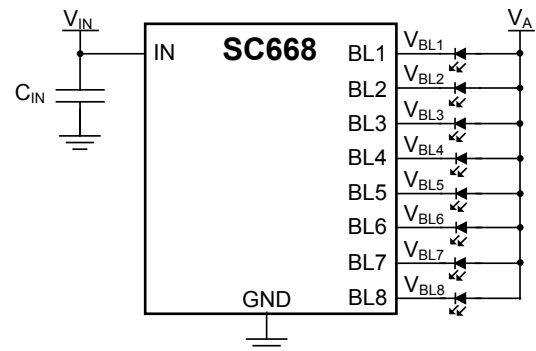
Figure 1 — Anode Supply
