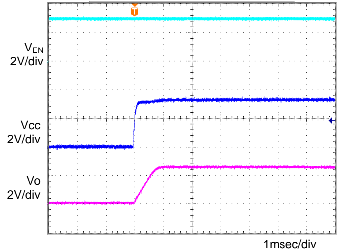
Figure 10. Input sequence 1 C_o=1\mu F, T_a=25^\circ C
