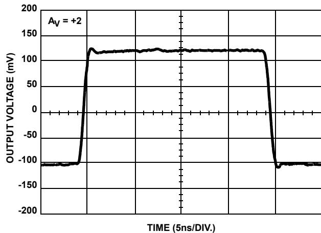
FIGURE 5. SMALL SIGNAL PULSE RESPONSE
