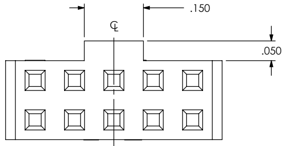
FIG 3 ISDM-05-K SHOWN (DIFFERENT AS SHOWN, OTHERWISE SAME AS FIG 2)
