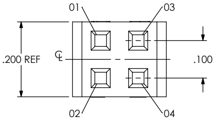
FIG 2 ISDM-02 SHOWN (DIFFERENT AS SHOWN, OTHERWISE SAME AS FIG 1)
