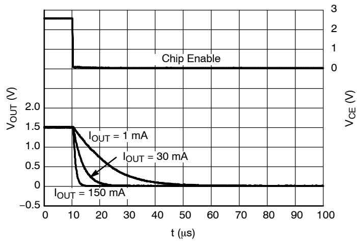
Figure 38. Shutdown, 1.5 V Version NCP4681D, V_{\text{IN}} = 2.5 \text{ V}
