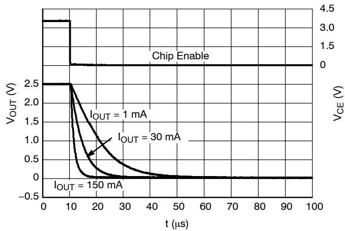
Figure 39. Shutdown, 2.5 V version NCP4681D, V_{\text{IN}} = 3.5 \text{ V}
