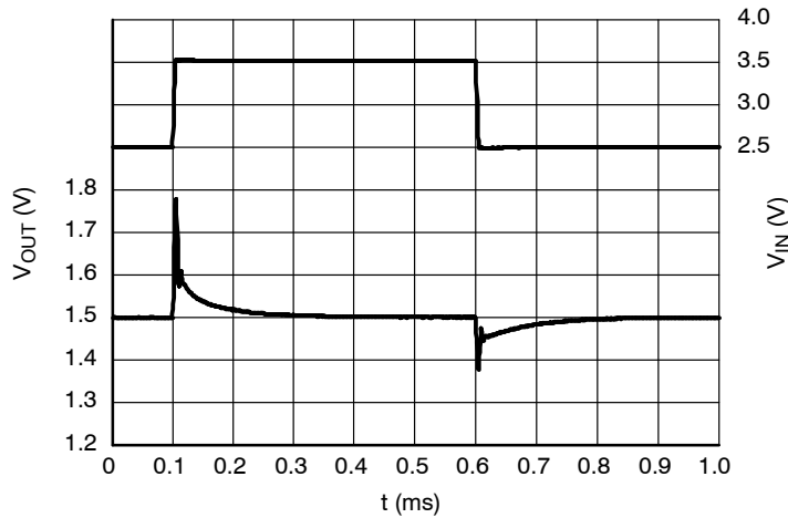
Figure 23. Line Transients, 1.5 V Version, t_R = t_F = 5 \mu\text{s} , I_{OUT} = 30 \text{ mA}
