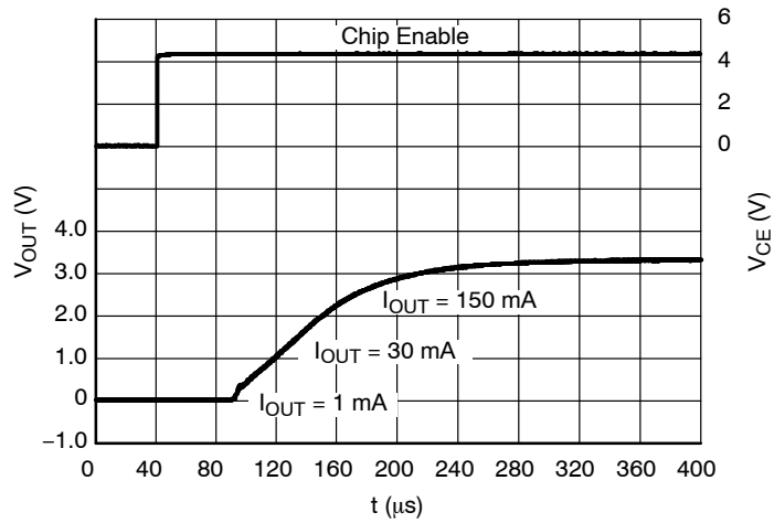
Figure 37. Start-up, 3.3 V Version NCP4681x, V_{\text{IN}} = 4.3 \text{ V}
