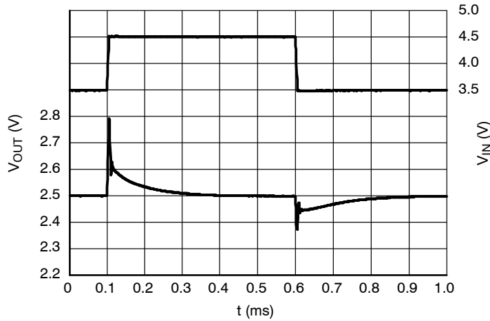
Figure 24. Line Transients, 2.5 V Version, t_R = t_F = 5 \mu\text{s} , I_{OUT} = 30 \text{ mA}
