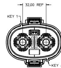
POLARIZATION "A"
