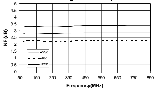
Noise Figure vs Temp
