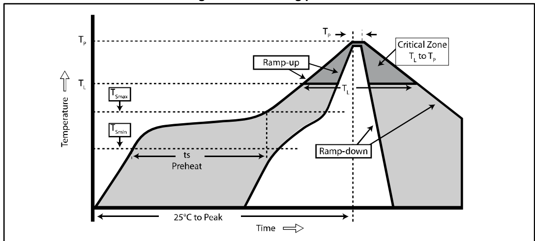
Figure 15: Soldering profiles
