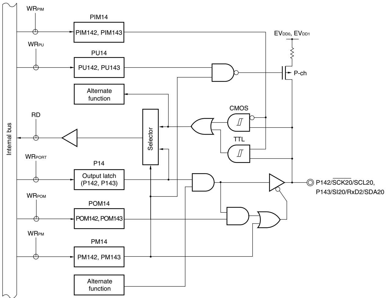
Figure 4-46. Block Diagram of P142 and P143
