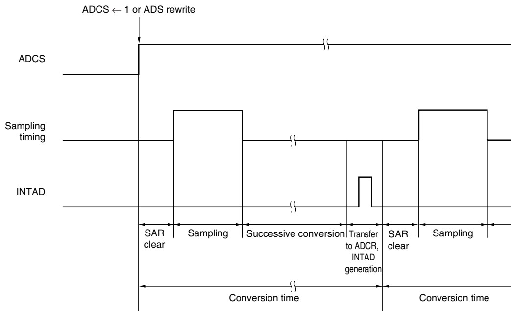
Figure 11-6. A/D Converter Sampling and A/D Conversion Timing
