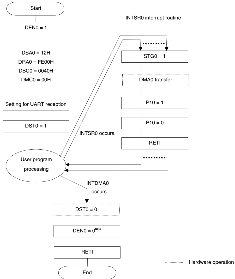
Figure 16-11. Setting Example of UART Consecutive Reception + ACK Transmission
