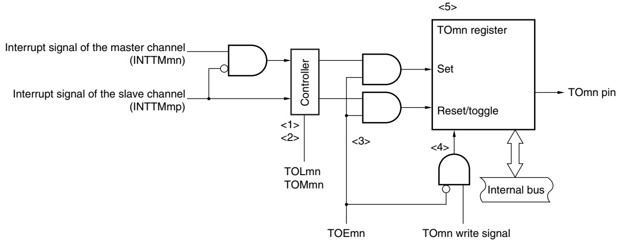
Figure 7-26. Output Circuit Configuration
