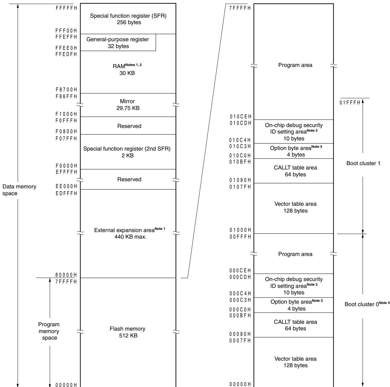
Figure 3-5. Memory Map ( \mu PD78F1178, 78F1178A)
