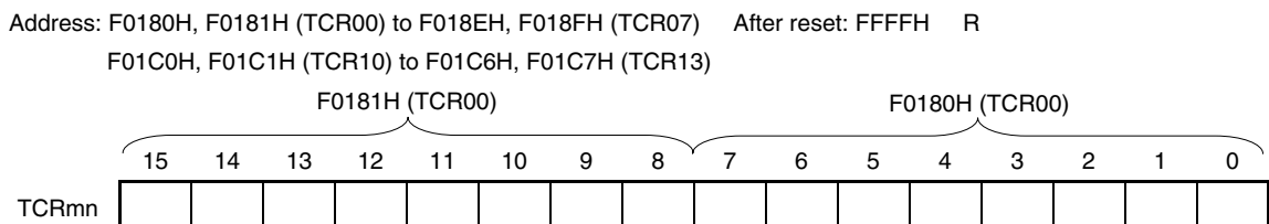
Figure 7-3. Format of Timer/Counter Register mn (TCRmn)
