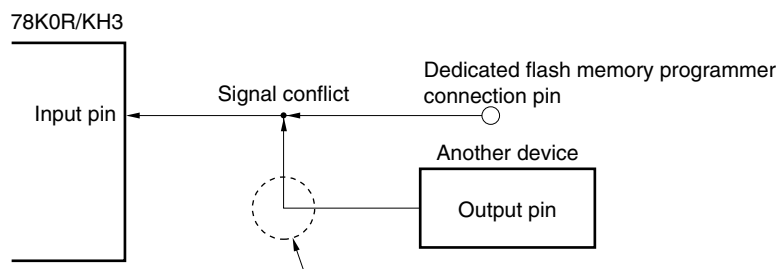
Figure 25-5. Signal Conflict ( \overline{\text{RESET}} Pin)
