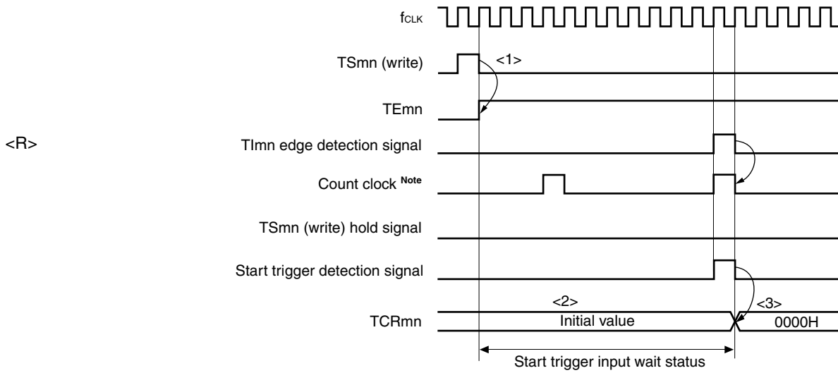
Figure 7-15. Start Timing (In Capture & One-count Mode)
