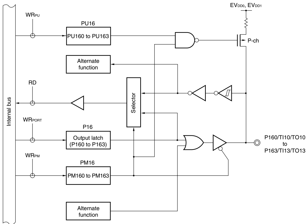
Figure 4-49. Block Diagram of P160 to P163
