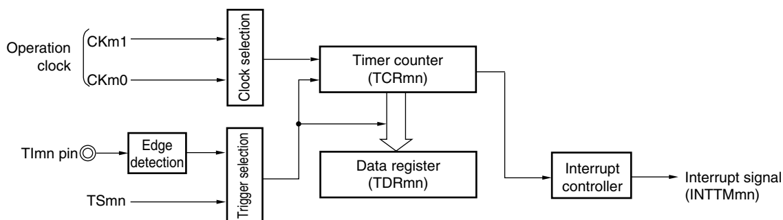
Figure 7-49. Block Diagram of Operation as Input Pulse Interval Measurement
