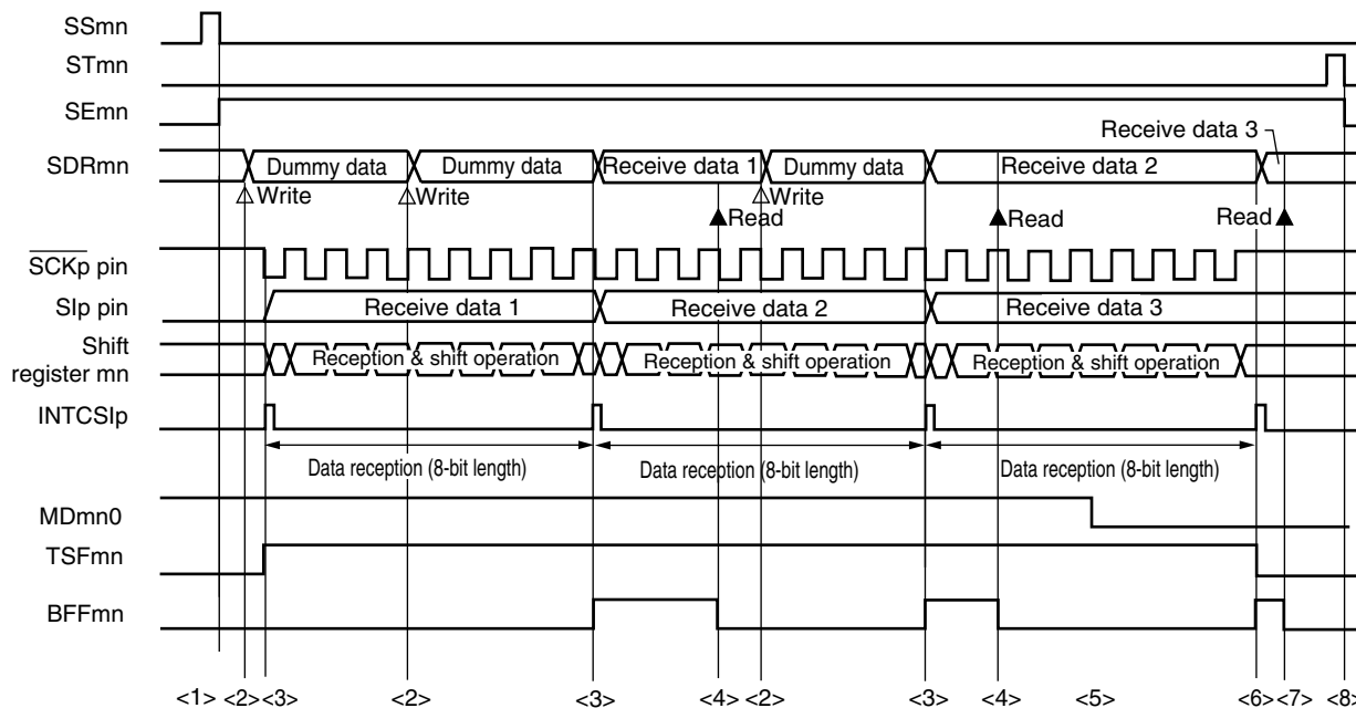
<R> Figure 13-38. Timing Chart of Master Reception (in Continuous Reception Mode) (Type 1: DAPmn = 0, CKPmn = 0)
