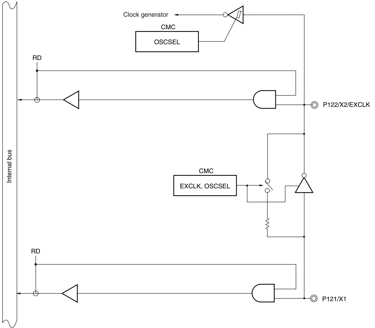
Figure 4-39. Block Diagram of P121 and P122
