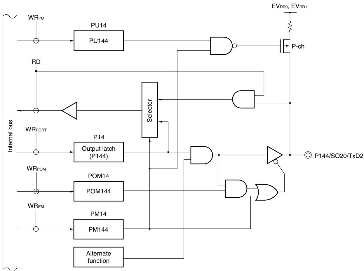
Figure 4-47. Block Diagram of P14
