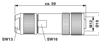
Dimensional drawing
