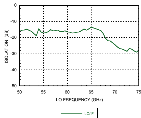
LO/IF Isolation
