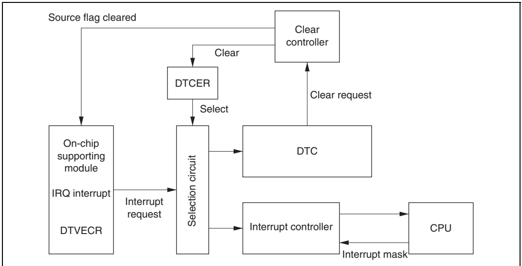
Figure 8.3 Block Diagram of DTC Activation Source Control
