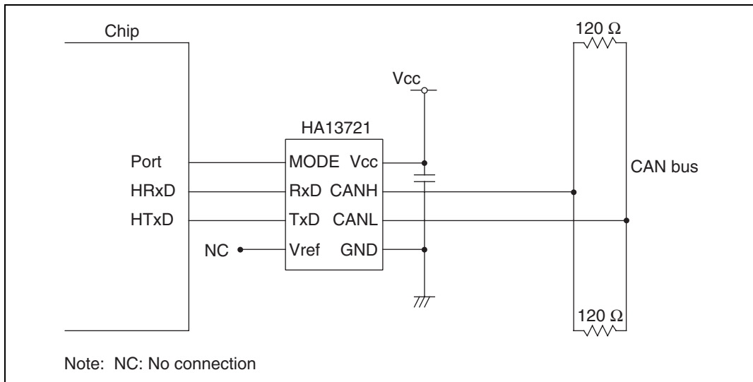
Figure 15.14 High-Speed Interface Using HA13721
