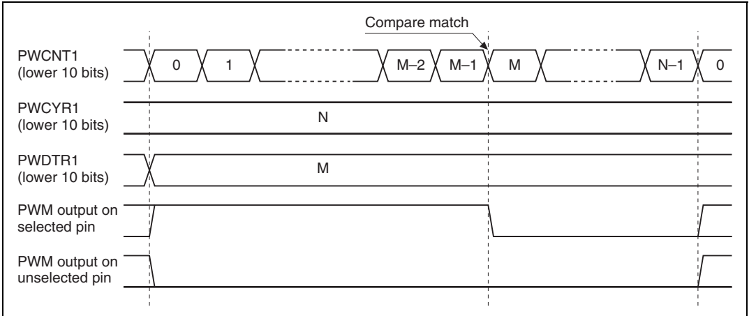
Figure 17.4 Duty Register Compare Match (OPS = 0 in PWPR1)
