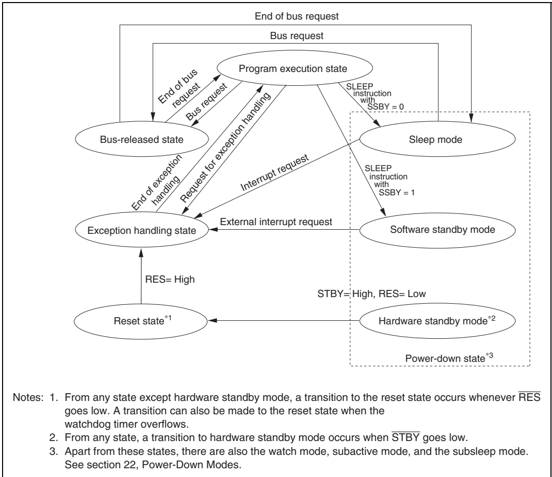
Figure 2.15 State Transitions
