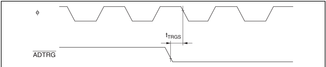
Figure 23.19 A/D Converter External Trigger Input Timing
