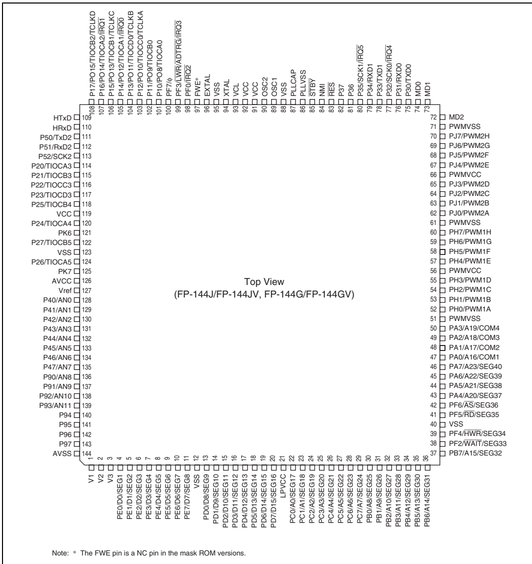
Figure 1.2 (2) H8S/2648, H8S/2648R, and H8S/2647 Pin Arrangement (FP-144J/FP-144JV, FP-144G/FP-144GV: Top View)
