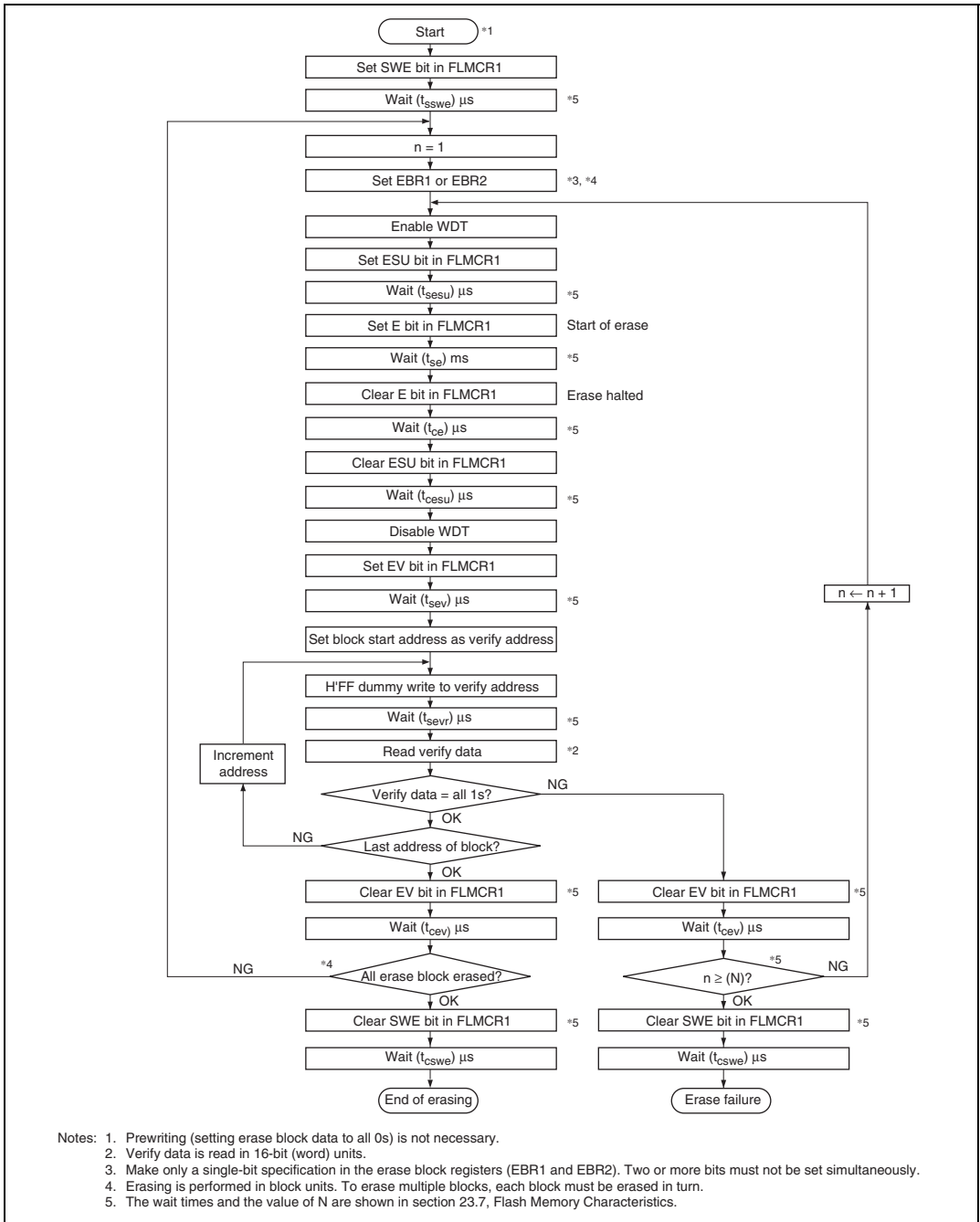
Figure 20.12 Erase/Erase-Verify Flowchart
