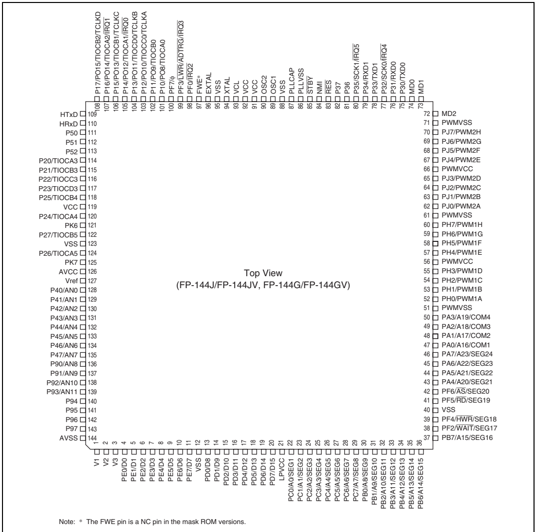
Figure 1.2 (1) H8S/2646, H8S/2646R, and H8S/2645 Pin Arrangement (FP-144J/FP-144JV, FP-144G/FP-144GV: Top View)
