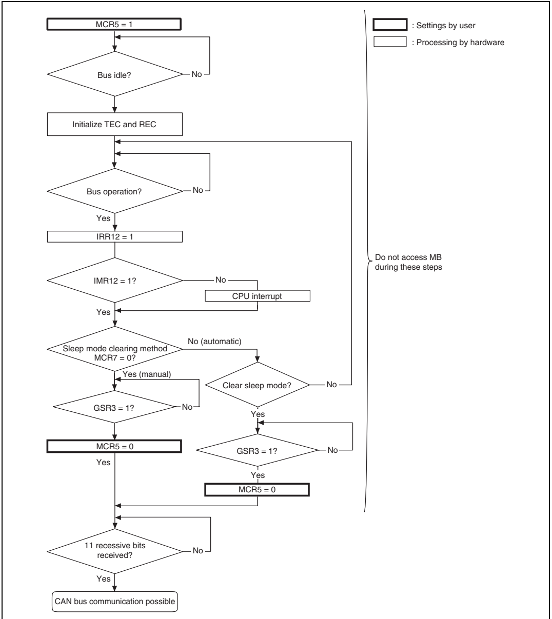
Figure 15.11 HCAN Sleep Mode Flowchart
