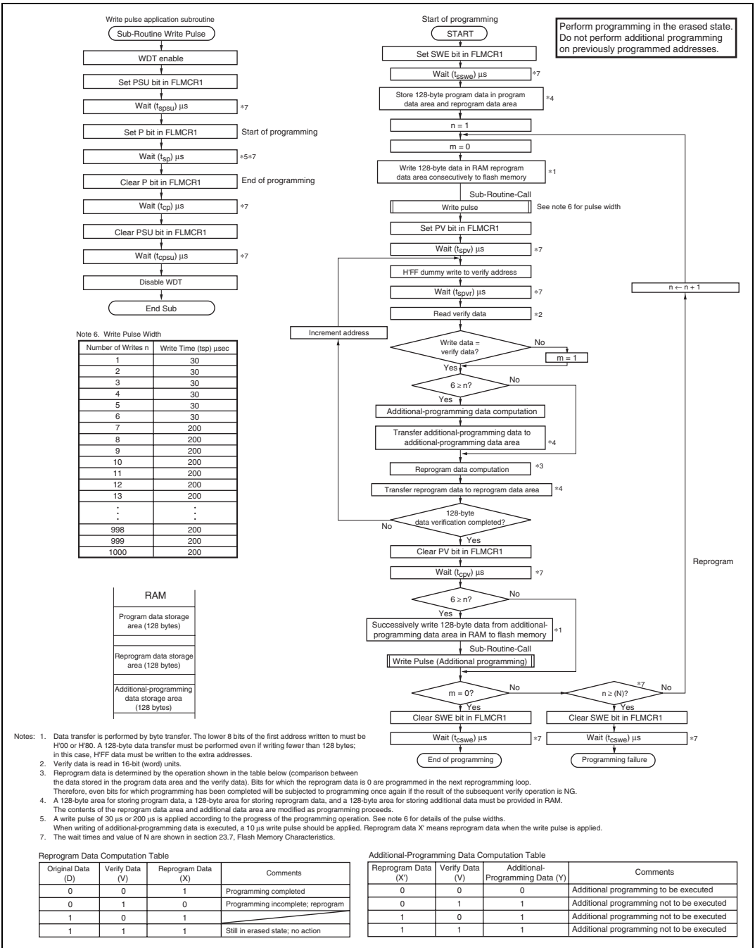
Figure 20.11 Program/Program-Verify Flowchart
