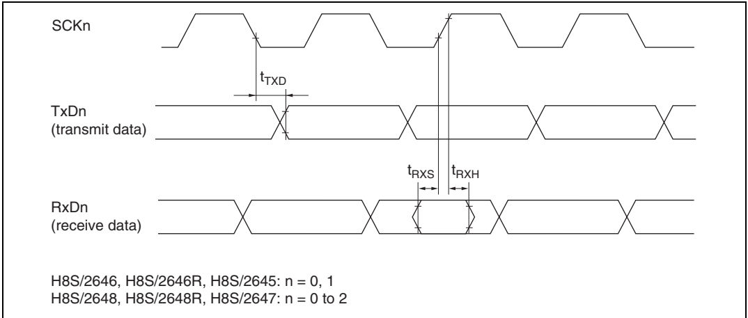
Figure 23.18 SCI Input/Output Timing (Clock Synchronous Mode)
