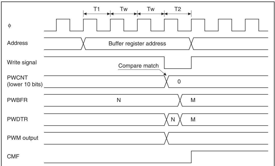
Figure 17.12 PWM Channel 1 Operation
