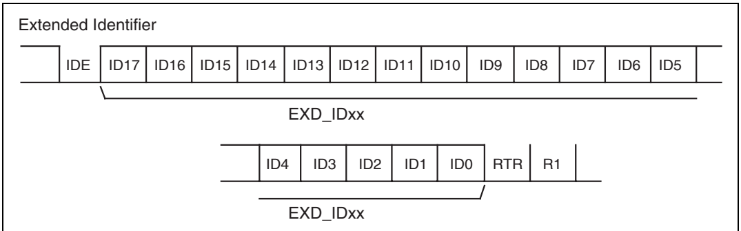
Figure 15.3 Extended Identifier
