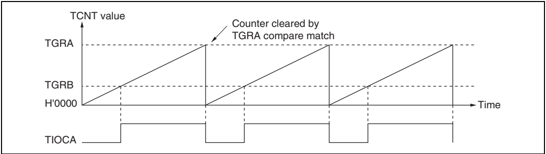
Figure 10.25 Example of PWM Mode Operation (1)
