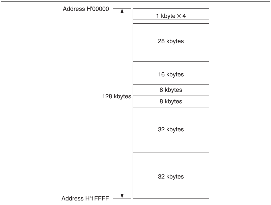
Figure 20.5 Block Configuration
