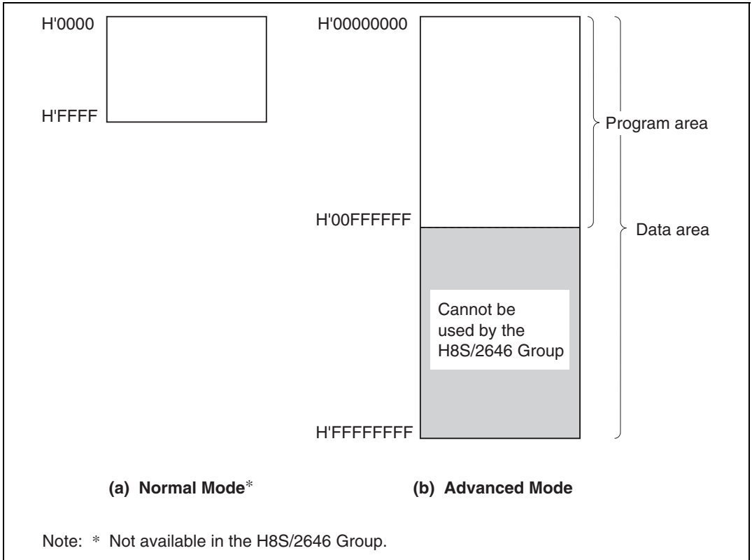
Figure 2.6 Memory Map
