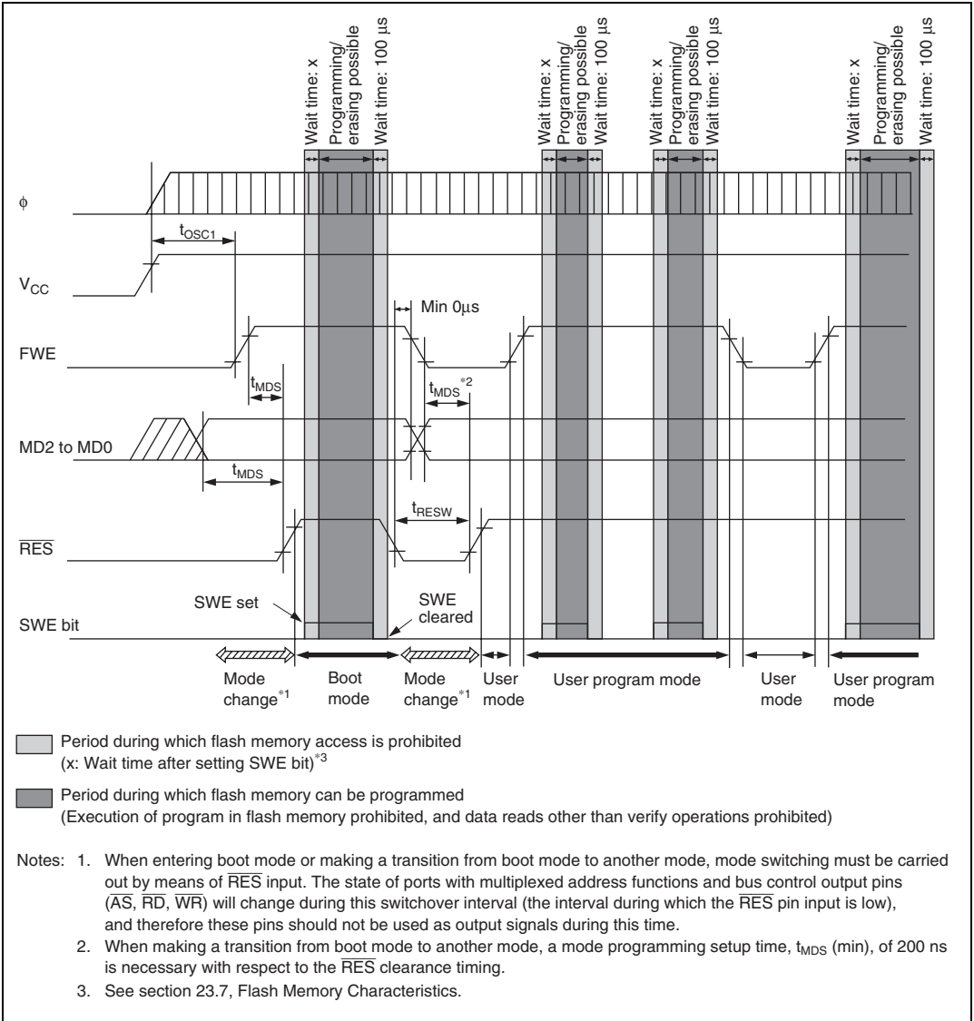
Figure 20.18 Mode Transition Timing (Example: Boot Mode → User Mode ↔ User Program Mode)
