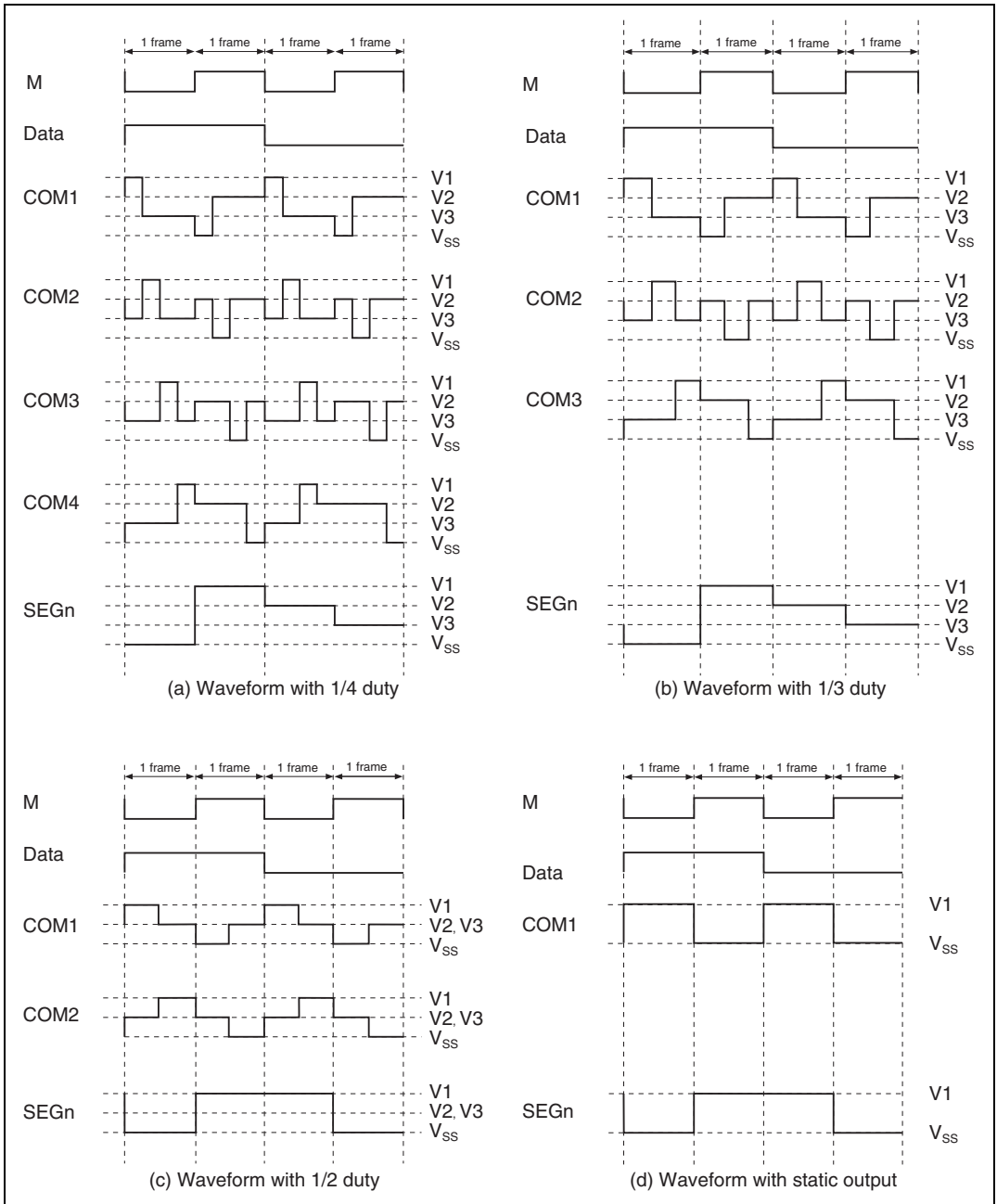
Figure 18.12 Output Waveforms for Each Duty Cycle (B Waveform)
