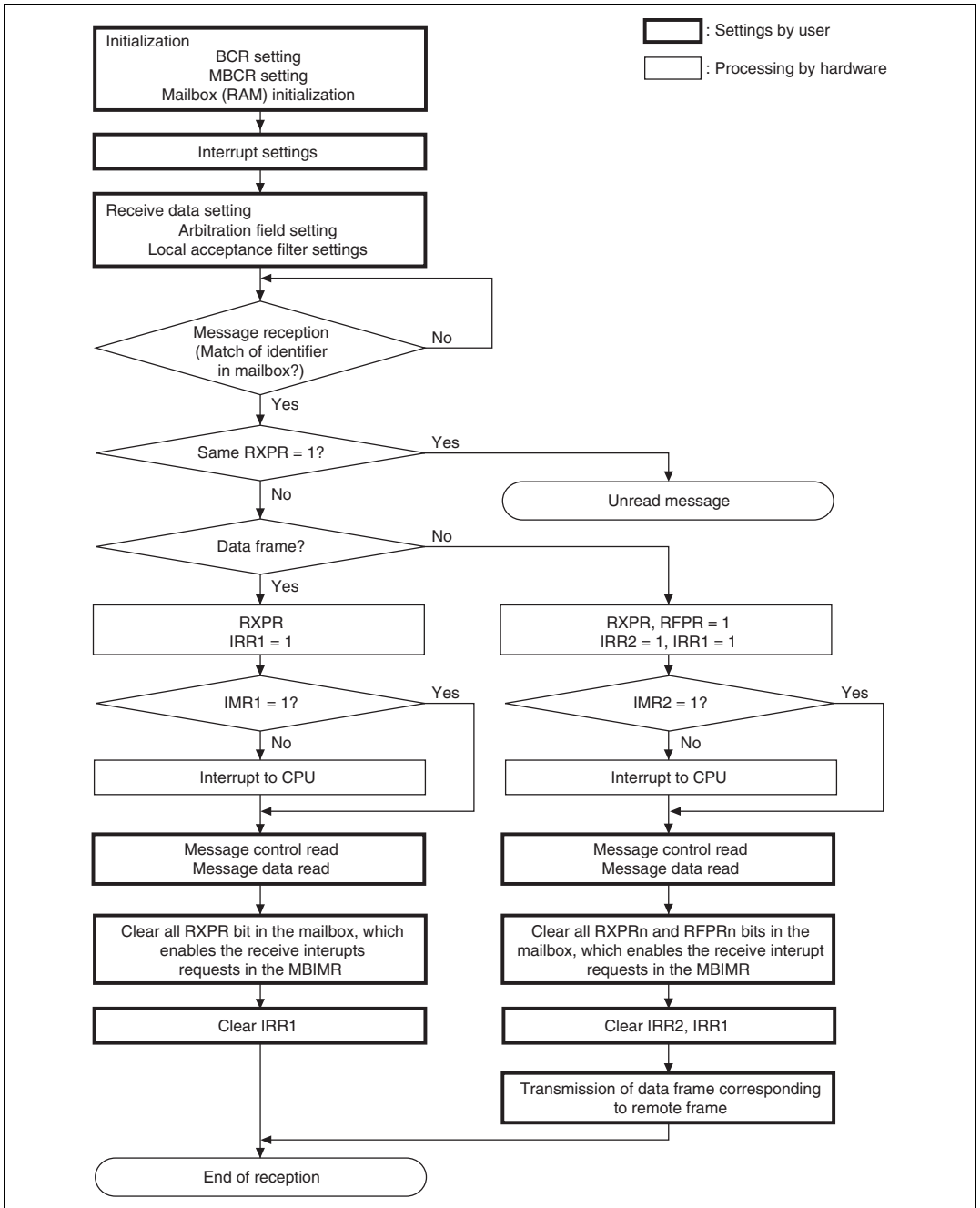
Figure 15.9 Reception Flowchart
