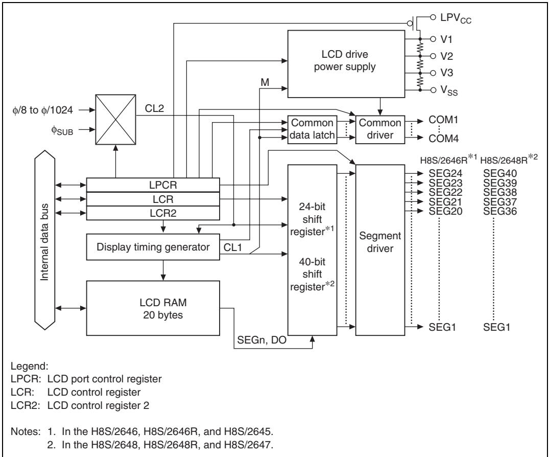
Figure 18.1 Block Diagram of LCD Controller/Driver
