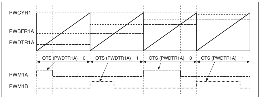
Figure 17.10 PWM Channel 1 Operation
