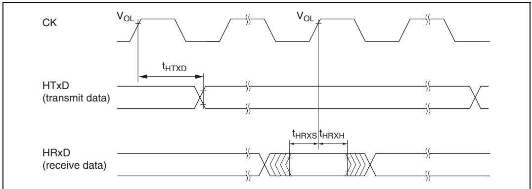
Figure 23.20 HCAN Input/Output Timing
