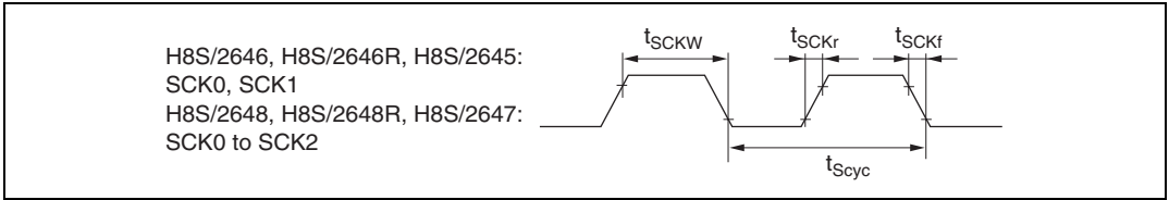
Figure 23.17 SCK Clock Input Timing
