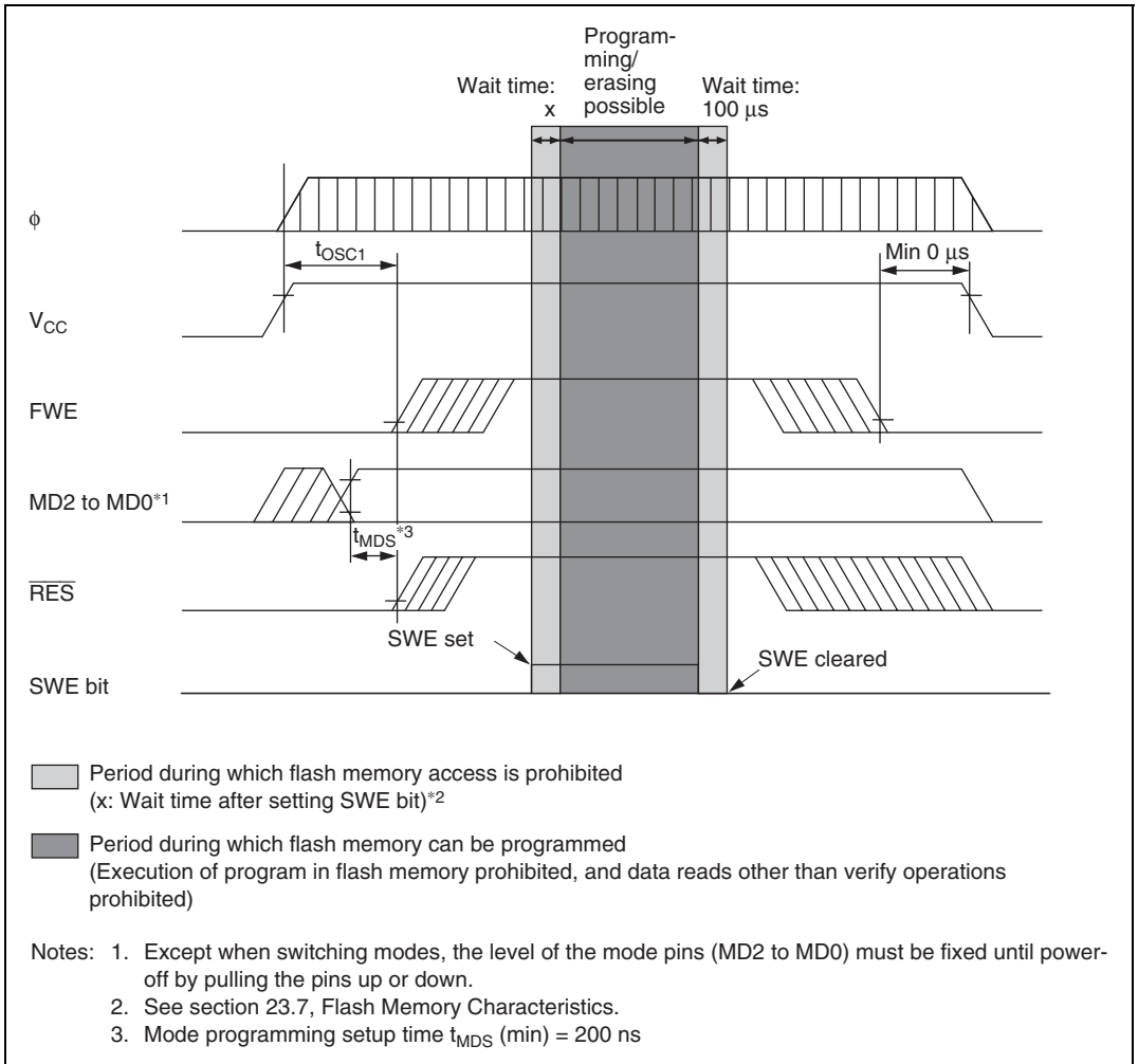
Figure 20.17 Power-On/Off Timing (User Program Mode)
