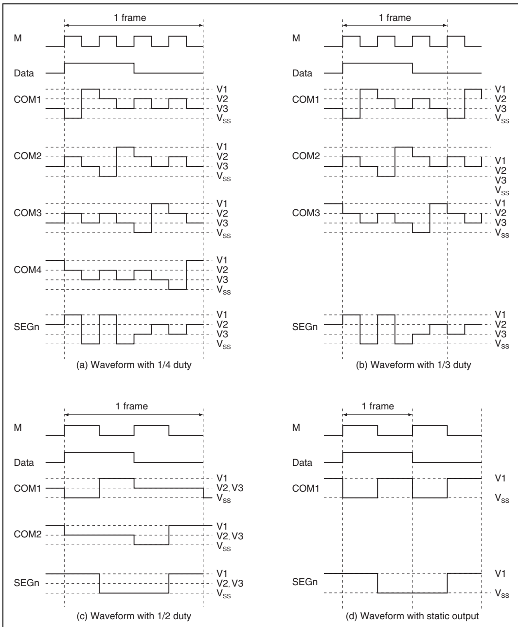
Figure 18.11 Output Waveforms for Each Duty Cycle (A Waveform)
