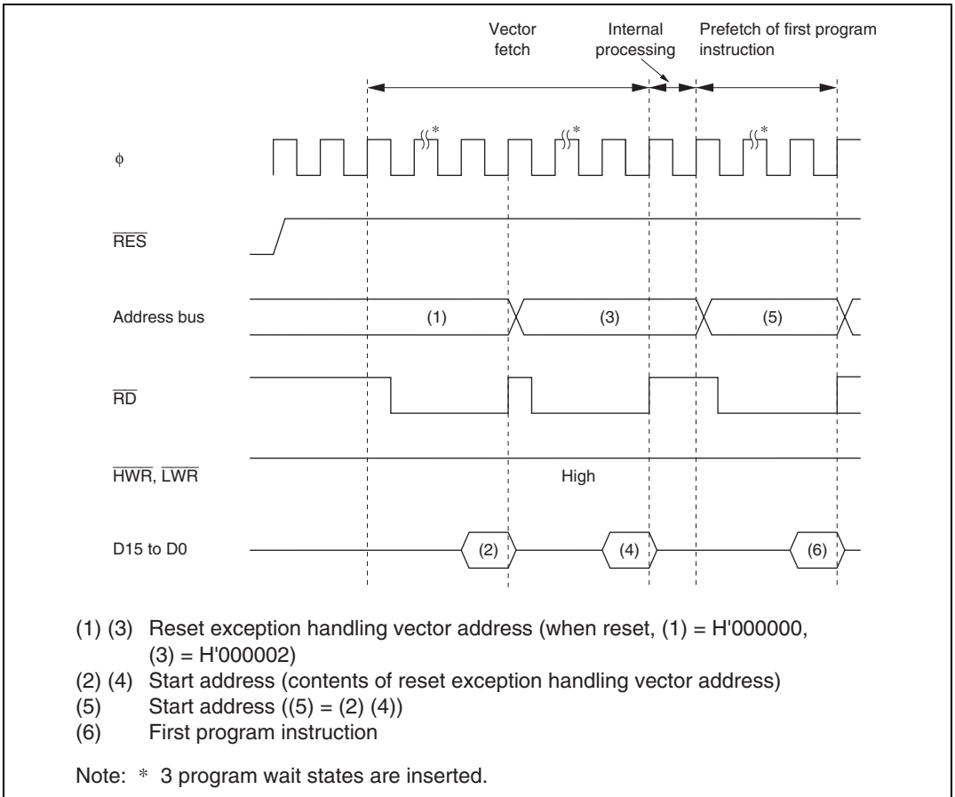
Figure 4.3 Reset Sequence (Mode 4)
