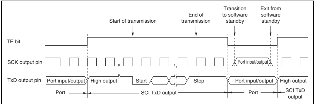
Figure 13.24 Asynchronous Transmission Using Internal Clock
