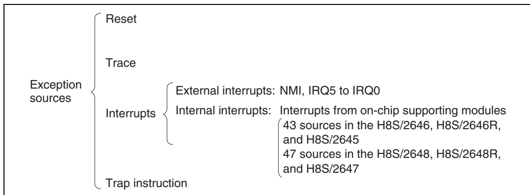
Figure 4.1 Exception Sources
