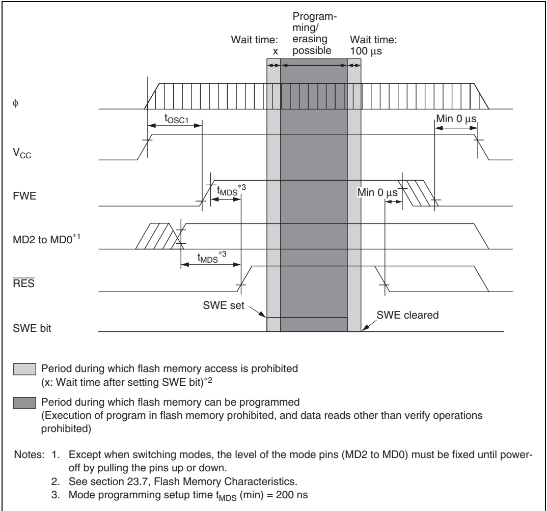
Figure 20.16 Power-On/Off Timing (Boot Mode)
