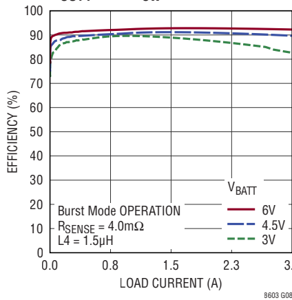
Channel 4 Efficiency vs Load V_{OUT4} = 8\text{V} , f_{SW} = 1.0\text{MHz}
