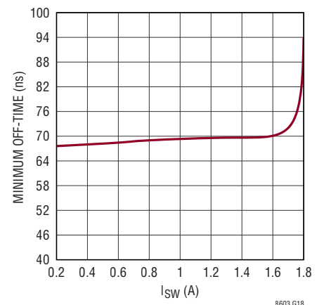
Channel 3 Minimum Off-Time vs I_{SW}
