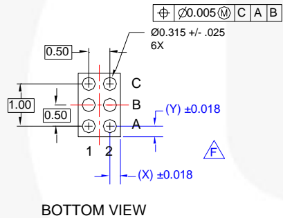
Figure 35. 6 Ball, 1.0 x 1.5 mm Wafer-Level Chip-Scale Packaging (WLCSP)
