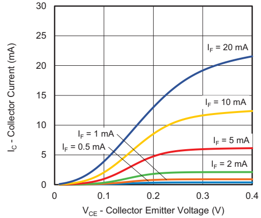
Fig. 10 - Collector Current vs. Collector Emitter Voltage (sat.)
