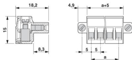
Dimensioned drawing
