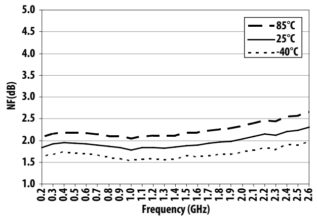
Figure 21. Noise Figure over Frequency and Temperature
