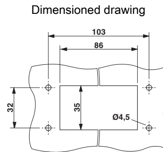
Panel cutout
