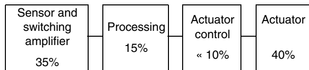
Figure 5 Safety loop
