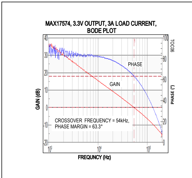
Figure 6. MAX17574 3.3V Output Full Load Bode Plot ( V_{IN} = 24V )
