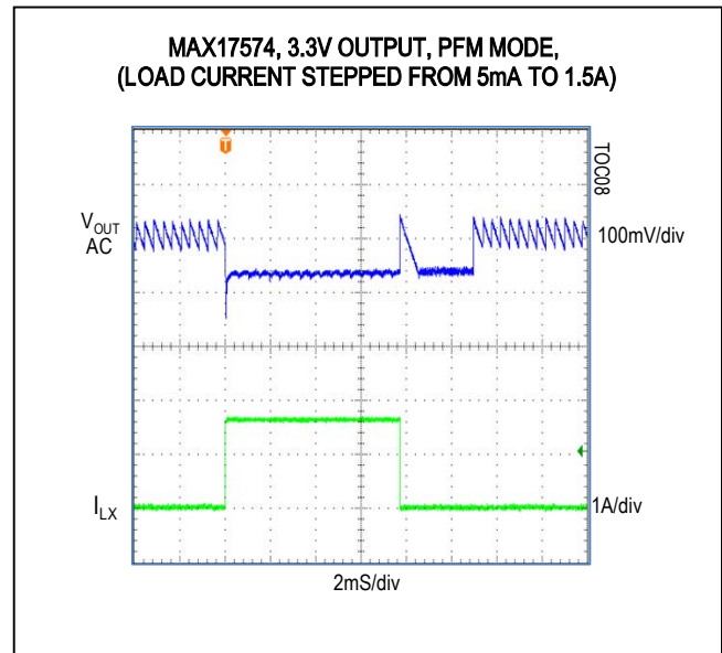
Figure 8. MAX17574 3.3V Output, 5mA to 1A Load Transient (PFM MODE/SYNC)
