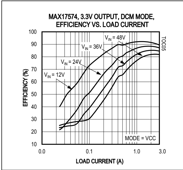
Figure 5. MAX17574 3.3V Output Efficiency (DCM MODE/SYNC)
