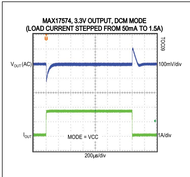
Figure 9. MAX17574 3.3V Output, 50mA to 1A Load Transient (DCM MODE/SYNC)
