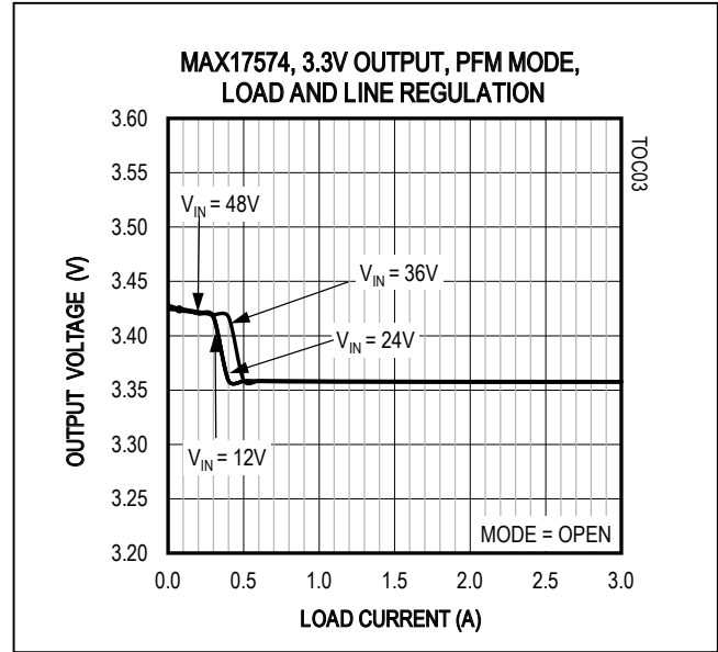
Figure 3. MAX17574 3.3V Output Load and Line Regulation (PFM MODE/SYNC)
