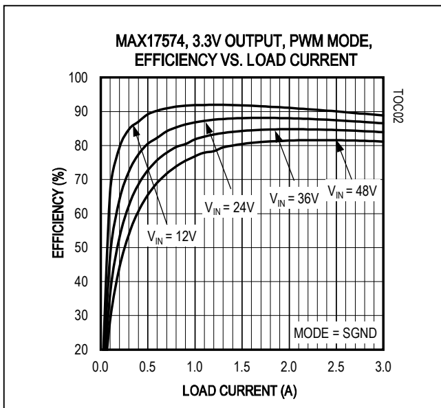
Figure 2. MAX17574 3.3V Output Efficiency (PWM MODE/SYNC)
