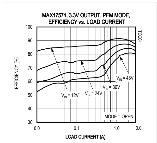
Figure 4. MAX17574 3.3V Output Efficiency (PFM MODE/SYNC)
