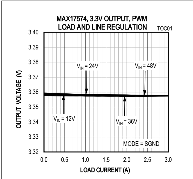
Figure 1. MAX17574 3.3V Output Load and Line Regulation (PWM MODE/SYNC)
