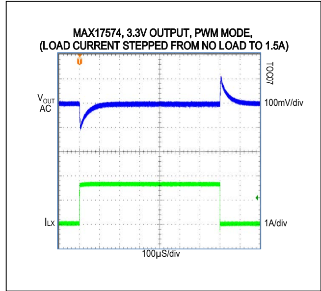
Figure 7. MAX17574 3.3V Output, No Load to 1A Load Transient (PWM MODE/SYNC)
