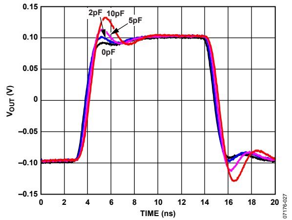
Figure 51. ADV3200 Small Signal Pulse with Capacitive Loads, 200 mV p-p
