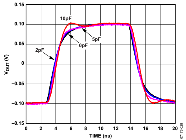
Figure 52. ADV3200 OSD Small Signal Pulse with Capacitive Loads, 200 mV p-p
