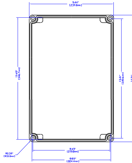
VIEW OF LID (INSIDE)
