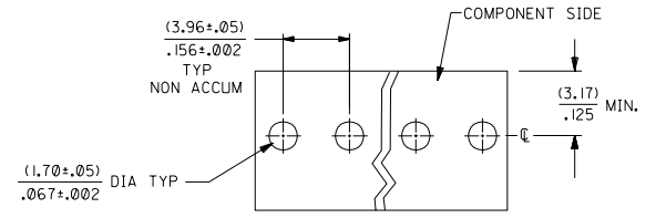
RECOMMENDED PC BOARD HOLE LAYOUT FOR CORRECT ORIENTATION OF PARTS WITH VOIDS ELIMINATE CORRESPONDING PCB HOLE
