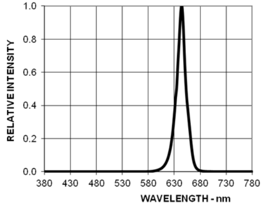
Figure 14 Relative Luminous Intensity Vs Wavelength
