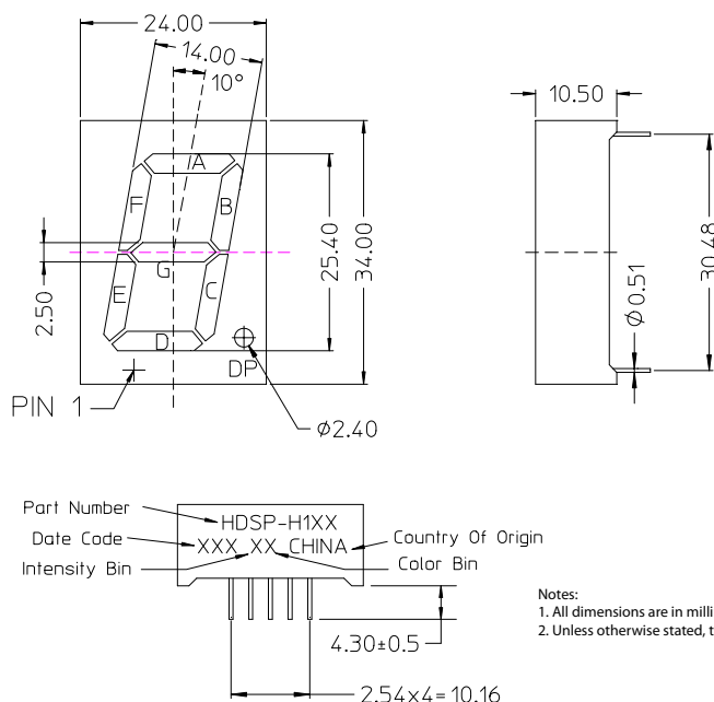
Figure 1 Package Dimension
