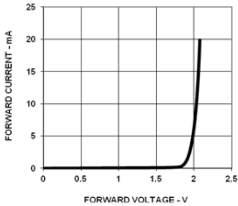
Figure 9 Forward Voltage Vs Current (DP)
