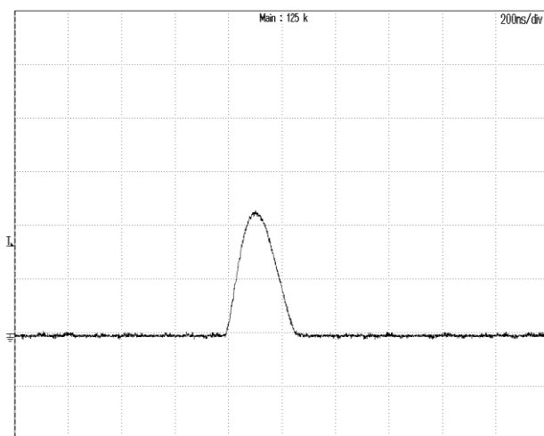
Figure 11: Inrush current @ Vin=72V CH1:lin, 2A/div, 200ns/div; Max current 4.3A, I2t=1.5E-7 A 2 S
