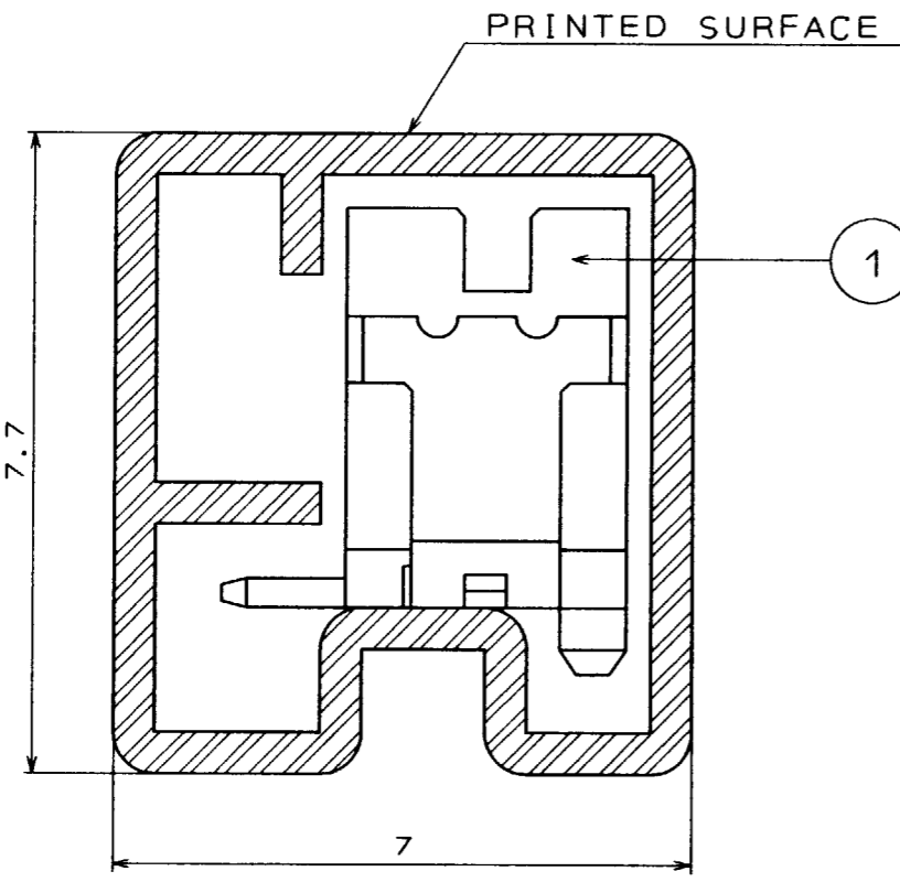
A-A SECTION(10/1)
