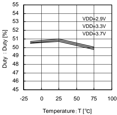
Fig.32 36.864MHz Temperature - Duty
