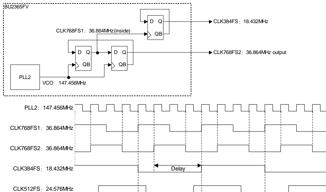
Fig.79 Audio Clock Output Circuit Configuration and Timing Chart
