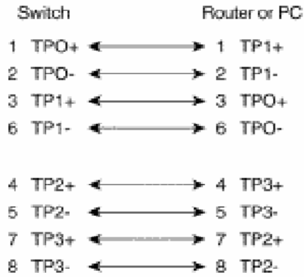
Straight through cables schematic
