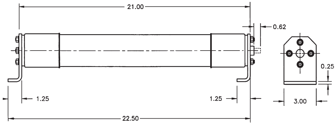
Figure 1 Dimensions - in
